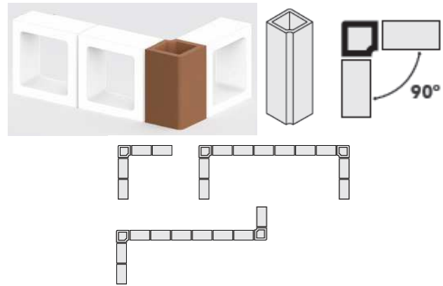
Corner Angle 90°
